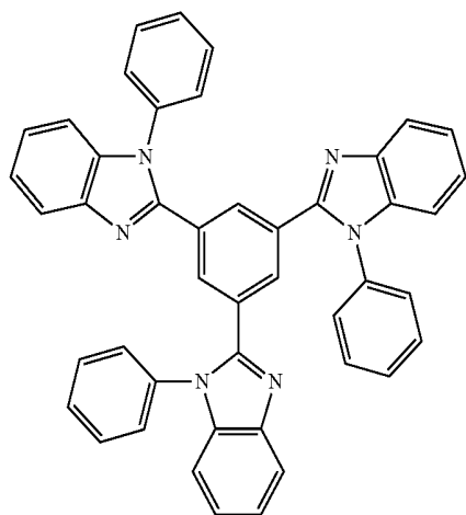
TPBI
